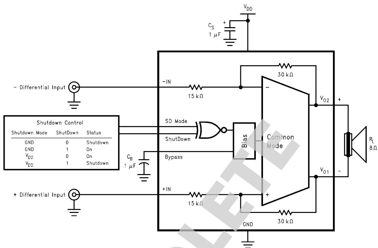
FIGURE 1. Typical Audio Amplifier Application Circuit
